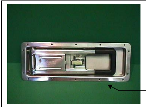
Combo Door Handle Part Number 811953 (Current Style)
